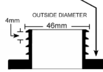
Thread Cutaway
