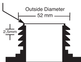
Thread Cutaway
