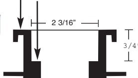
Thread Cutaway
